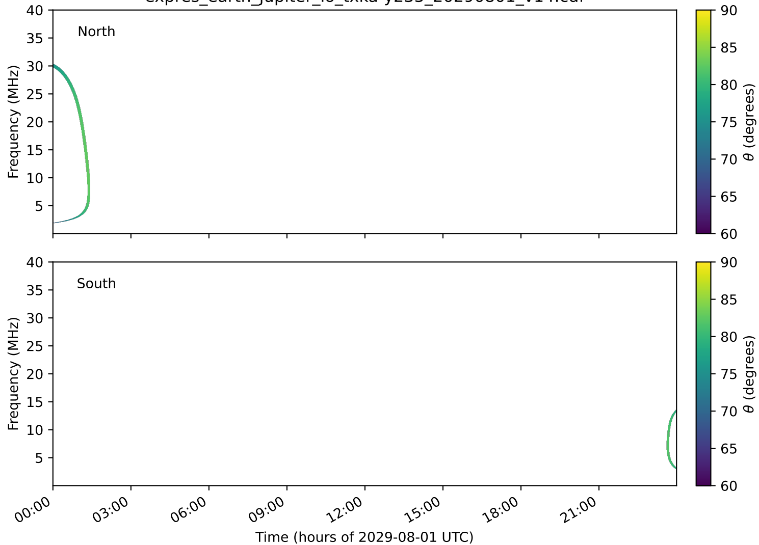
expres_earth_jupiter_io_txka-y235_20290801_v14.cdf
