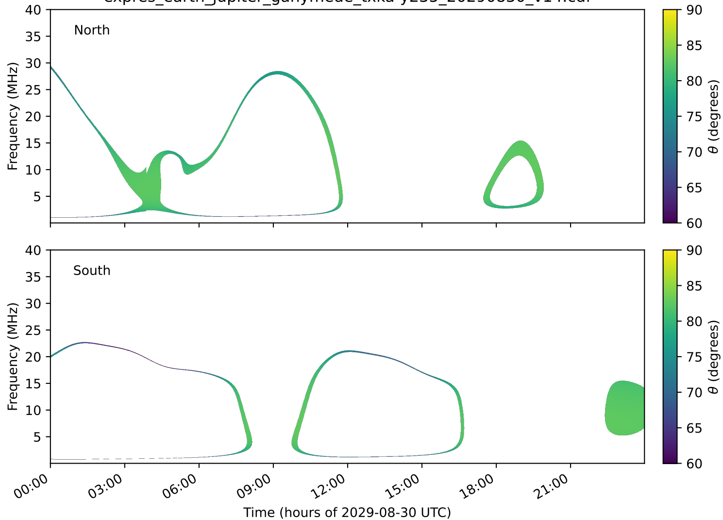
expres_earth_jupiter_ganymede_txka-y235_20290830_v14.cdf
