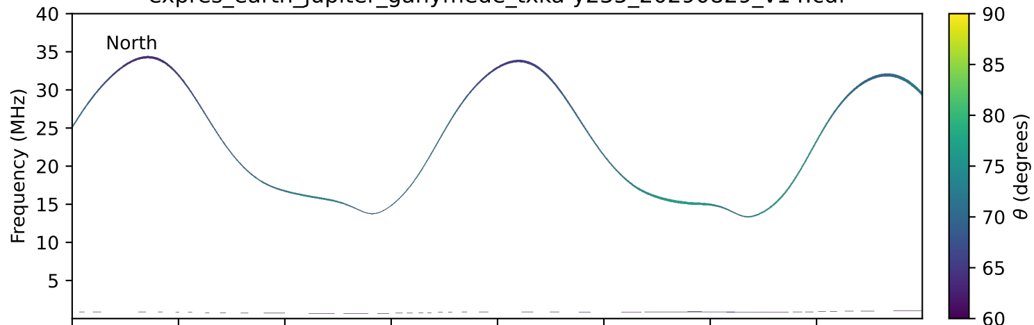
expres_earth_jupiter_ganymede_txka-y235_20290829_v14.cdf
