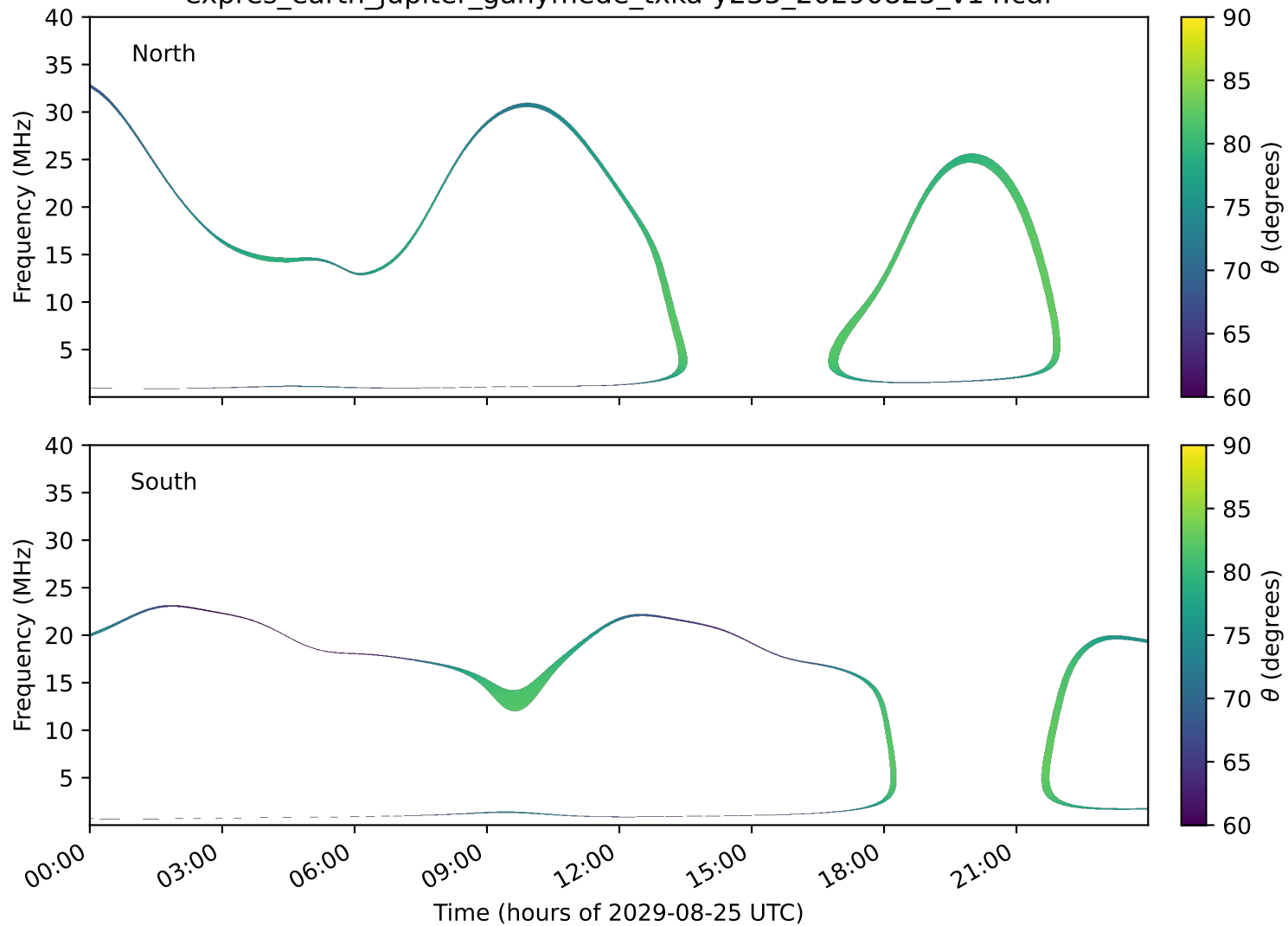
expres_earth_jupiter_ganymede_txka-y235_20290825_v14.cdf
