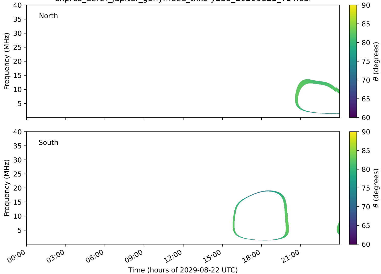
expres_earth_jupiter_ganymede_txka-y235_20290822_v14.cdf
