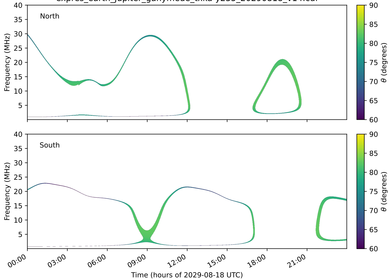
expres_earth_jupiter_ganymede_txka-y235_20290818_v14.cdf
