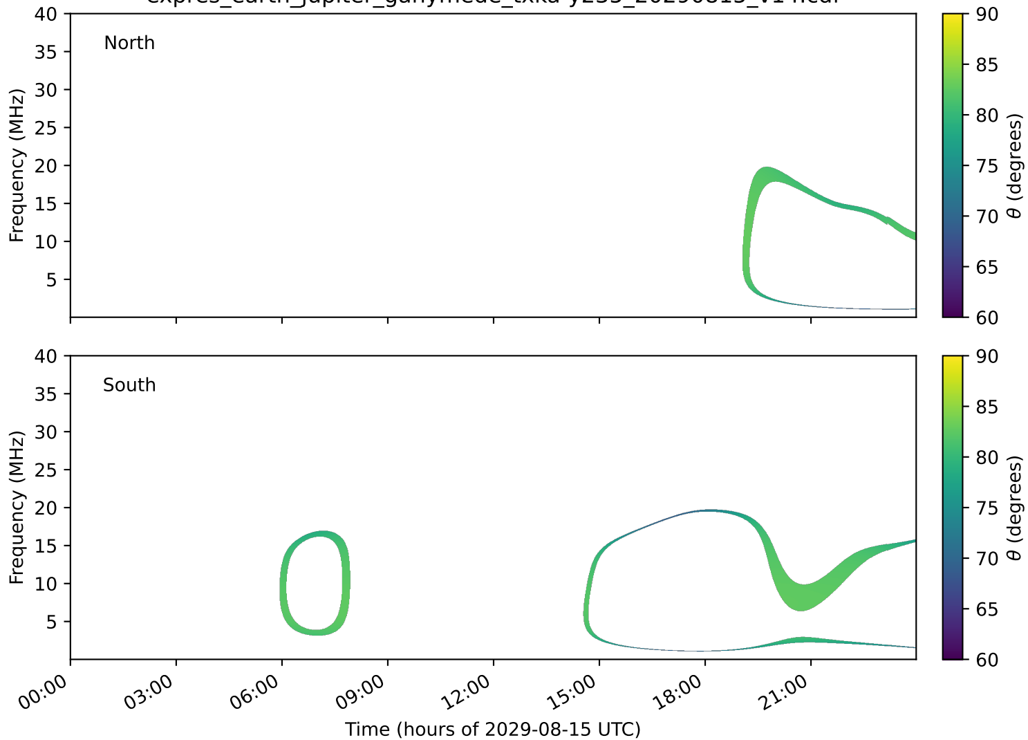
expres_earth_jupiter_ganymede_txka-y235_20290815_v14.cdf
