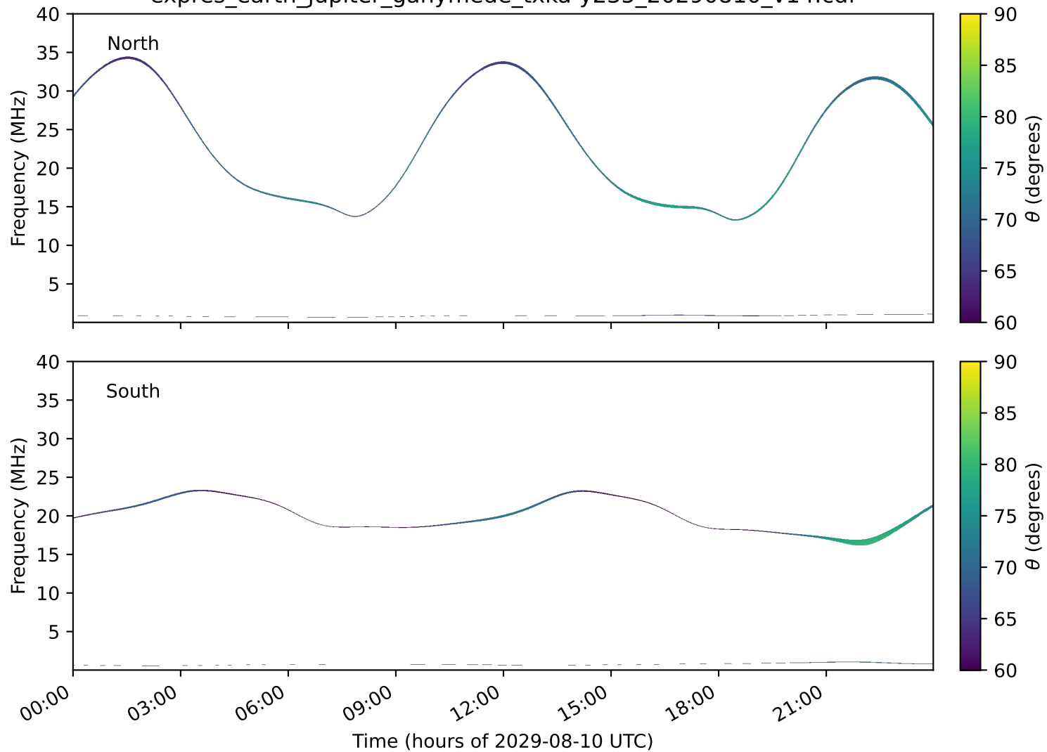
expres_earth_jupiter_ganymede_txka-y235_20290810_v14.cdf
