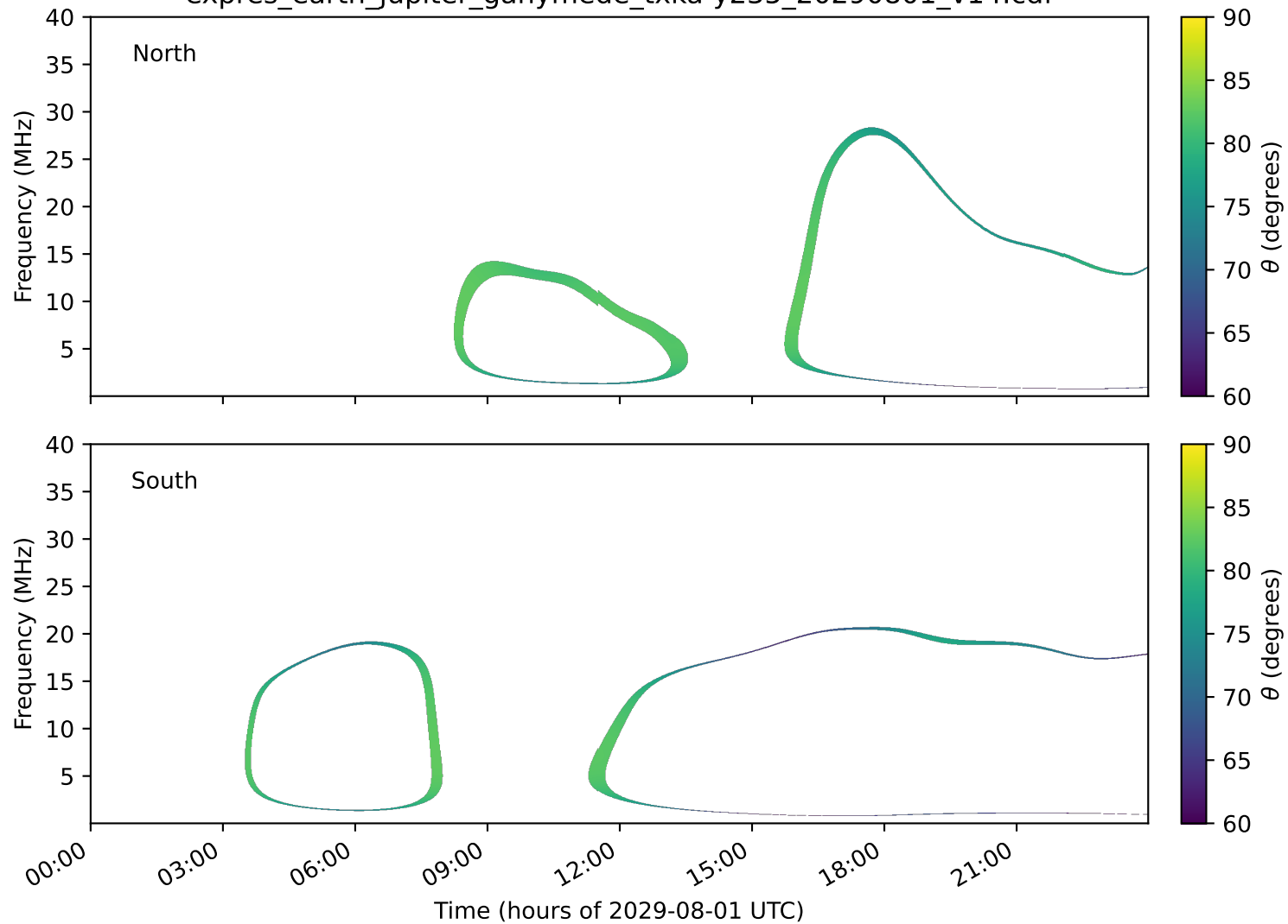
expres_earth_jupiter_ganymede_txka-y235_20290801_v14.cdf
