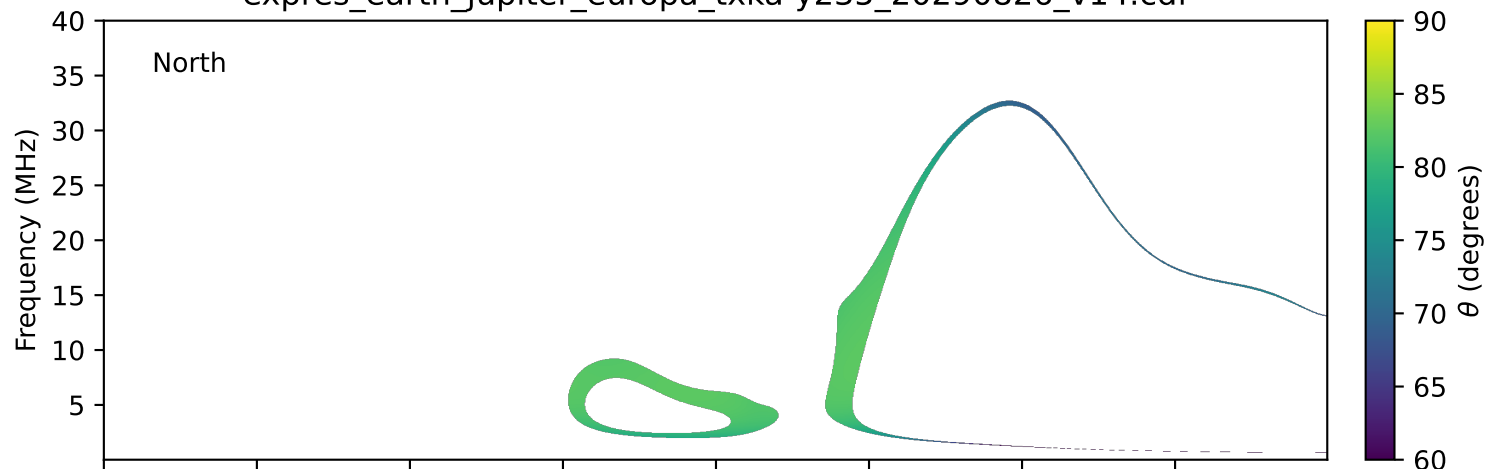
expres_earth_jupiter_europa_txka-y235_20290826_v14.cdf
