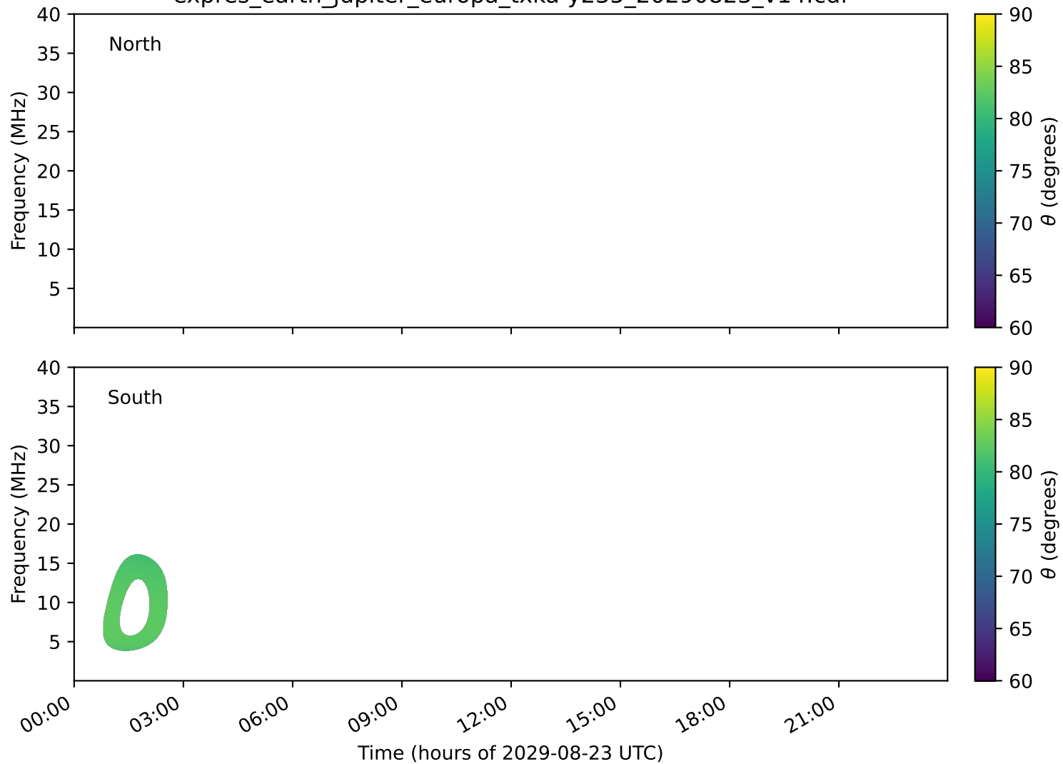
expres_earth_jupiter_europa_txka-y235_20290823_v14.cdf
