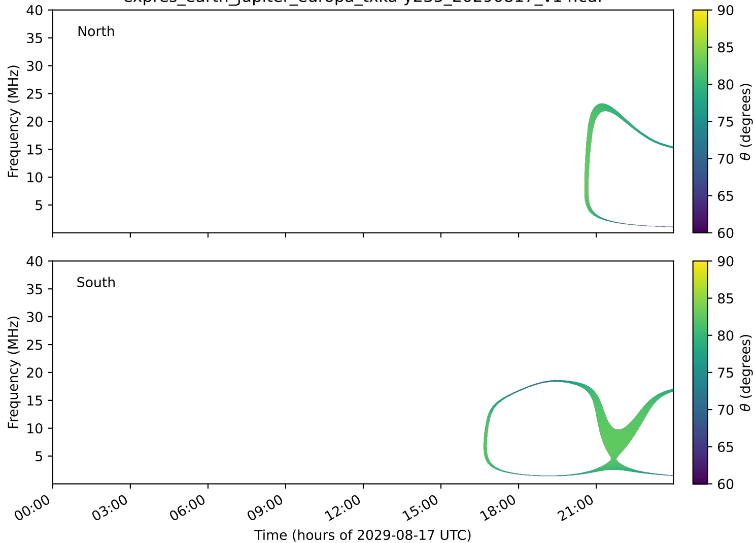
expres_earth_jupiter_europa_txka-y235_20290817_v14.cdf
