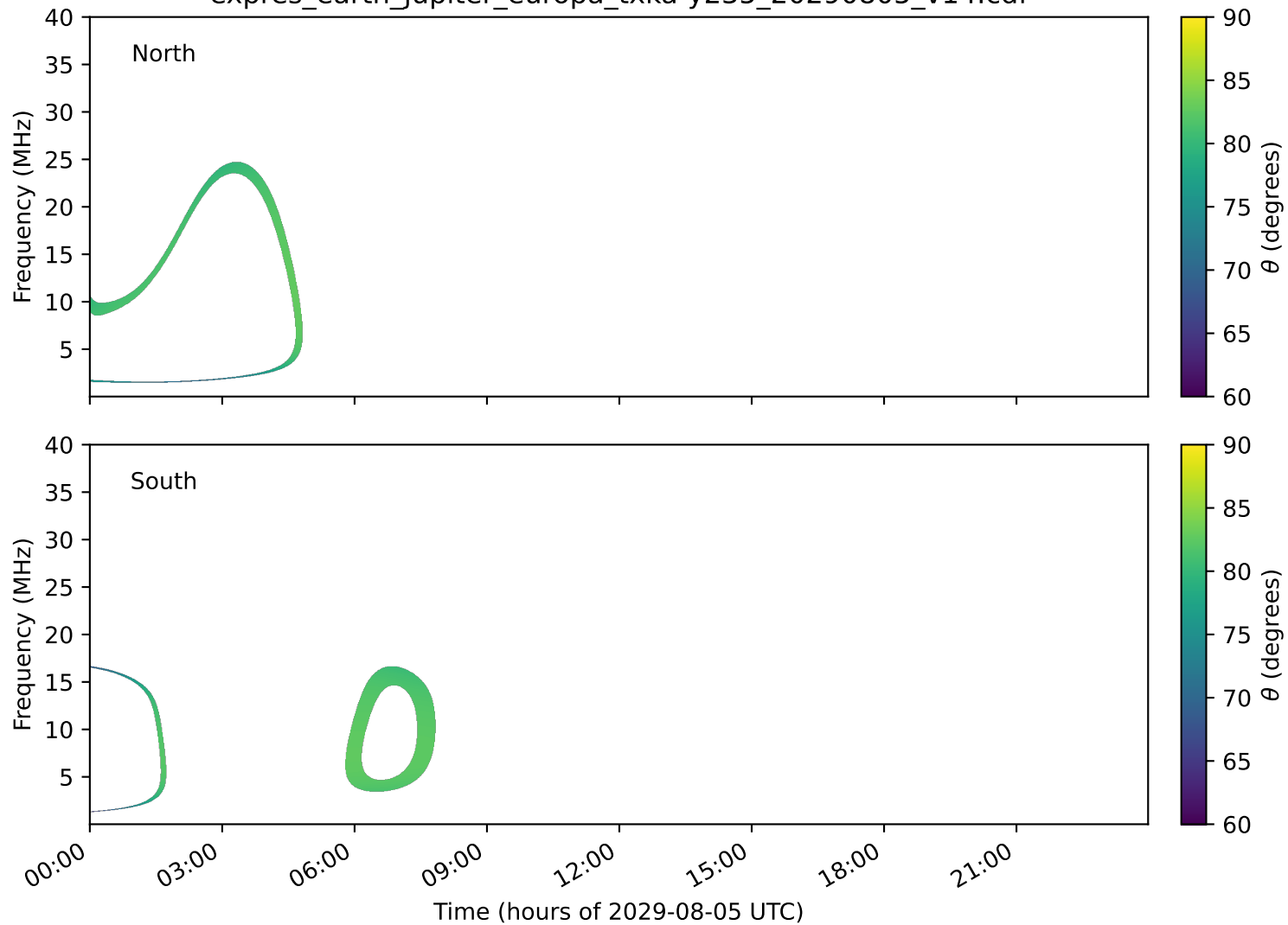
expres_earth_jupiter_europa_txka-y235_20290805_v14.cdf
