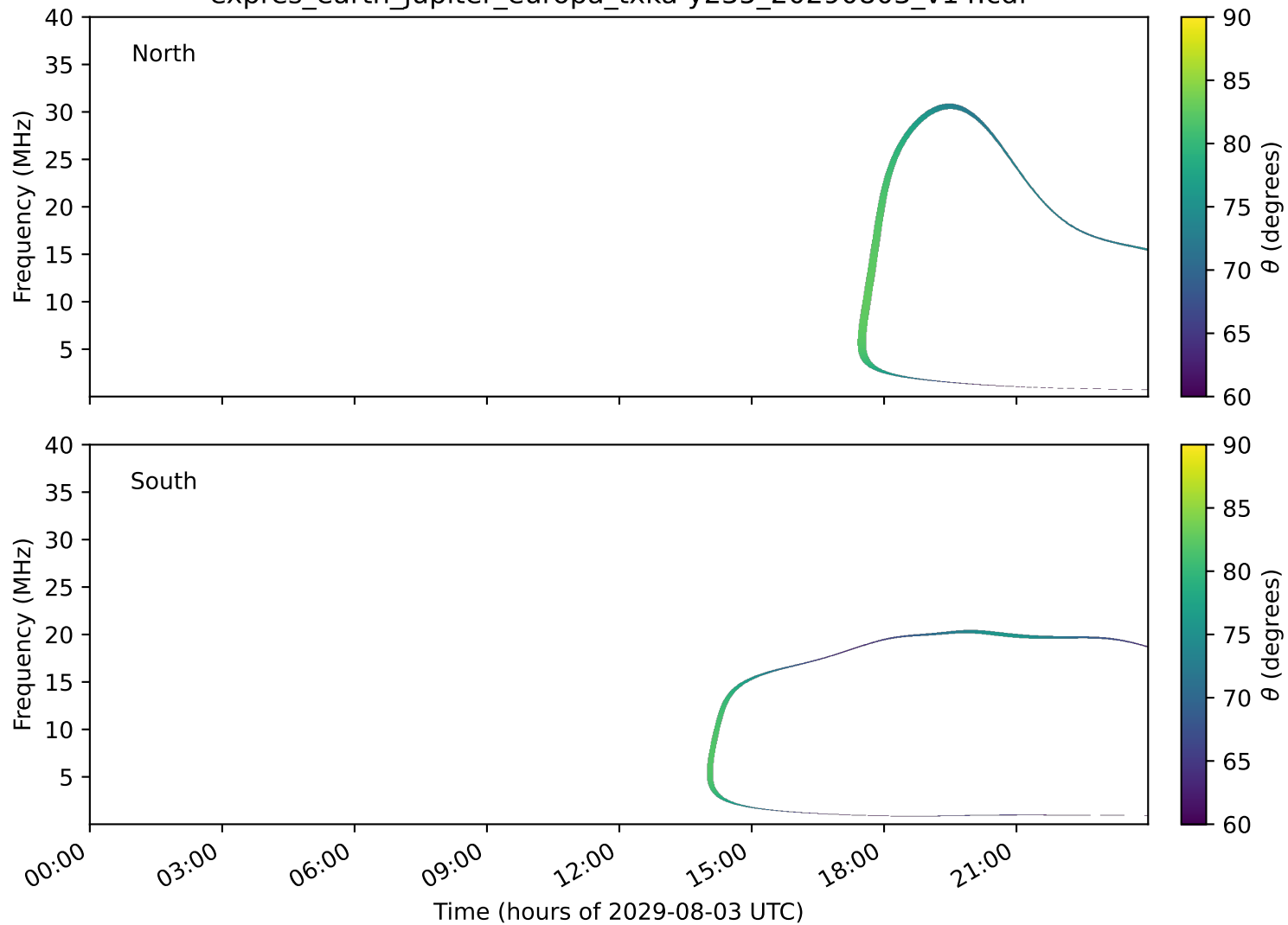
expres_earth_jupiter_europa_txka-y235_20290803_v14.cdf
