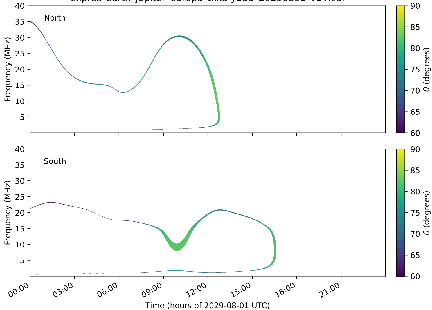
expres_earth_jupiter_europa_txka-y235_20290801_v14.cdf
