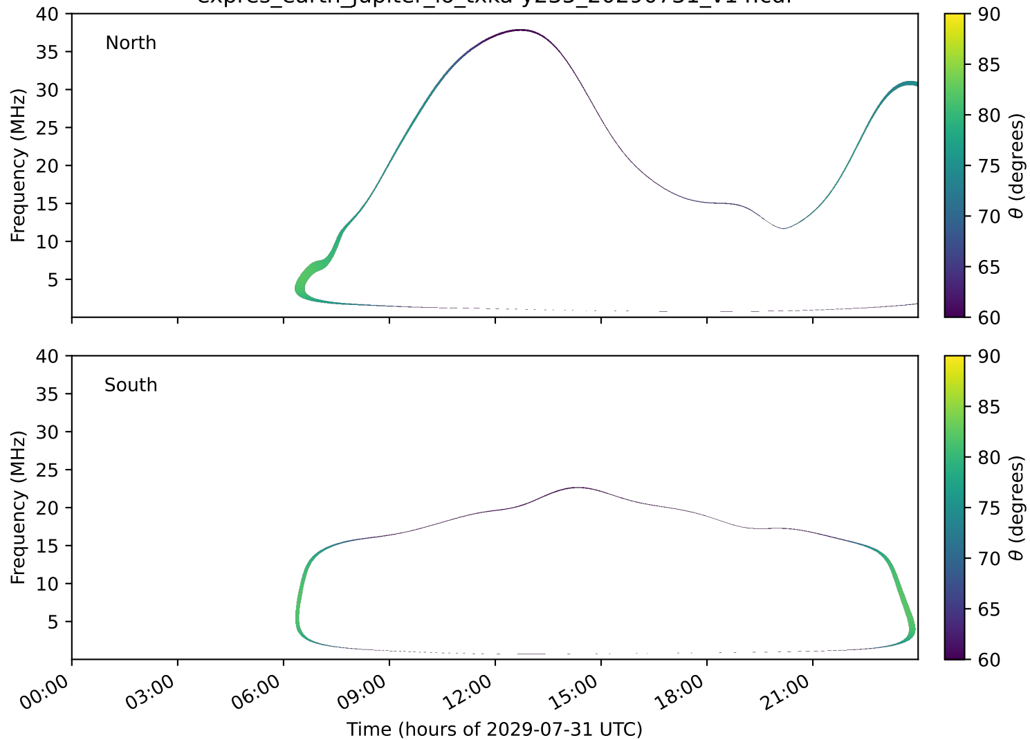
expres_earth_jupiter_io_txka-y235_20290731_v14.cdf
