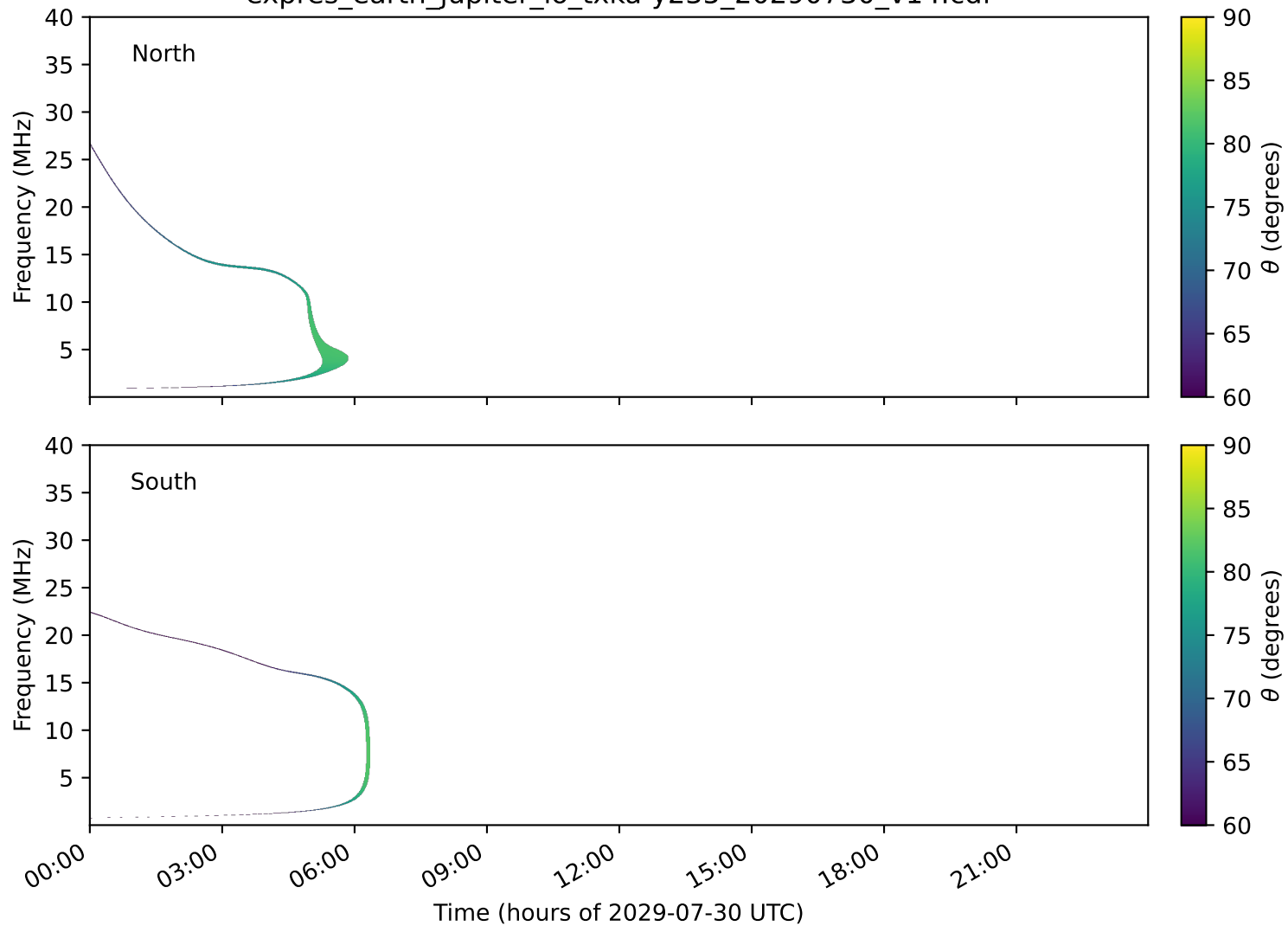
expres_earth_jupiter_io_txka-y235_20290730_v14.cdf
