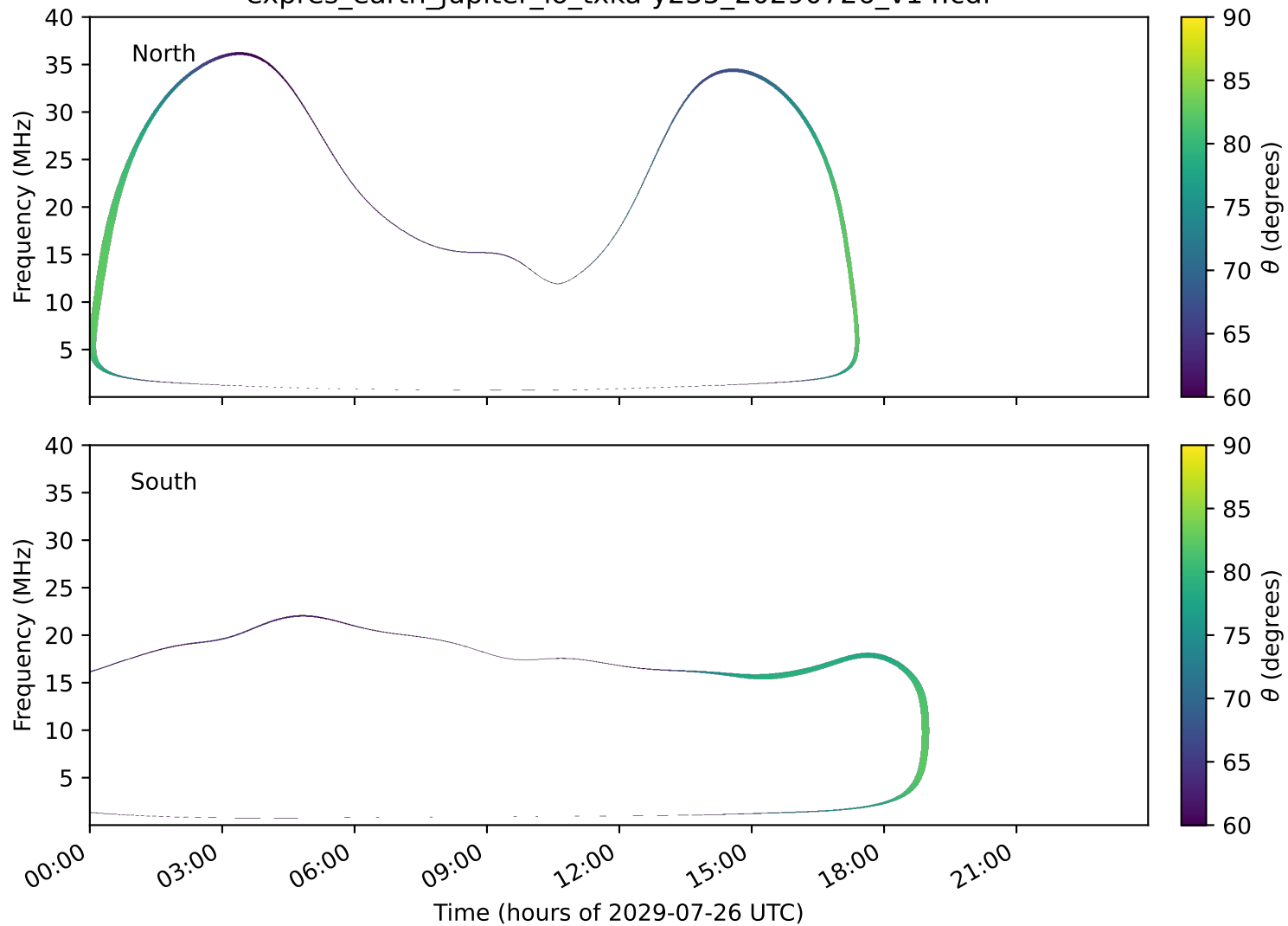
expres_earth_jupiter_io_txka-y235_20290726_v14.cdf
