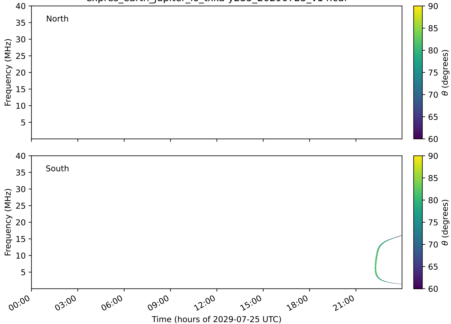
expres_earth_jupiter_io_txka-y235_20290725_v14.cdf
