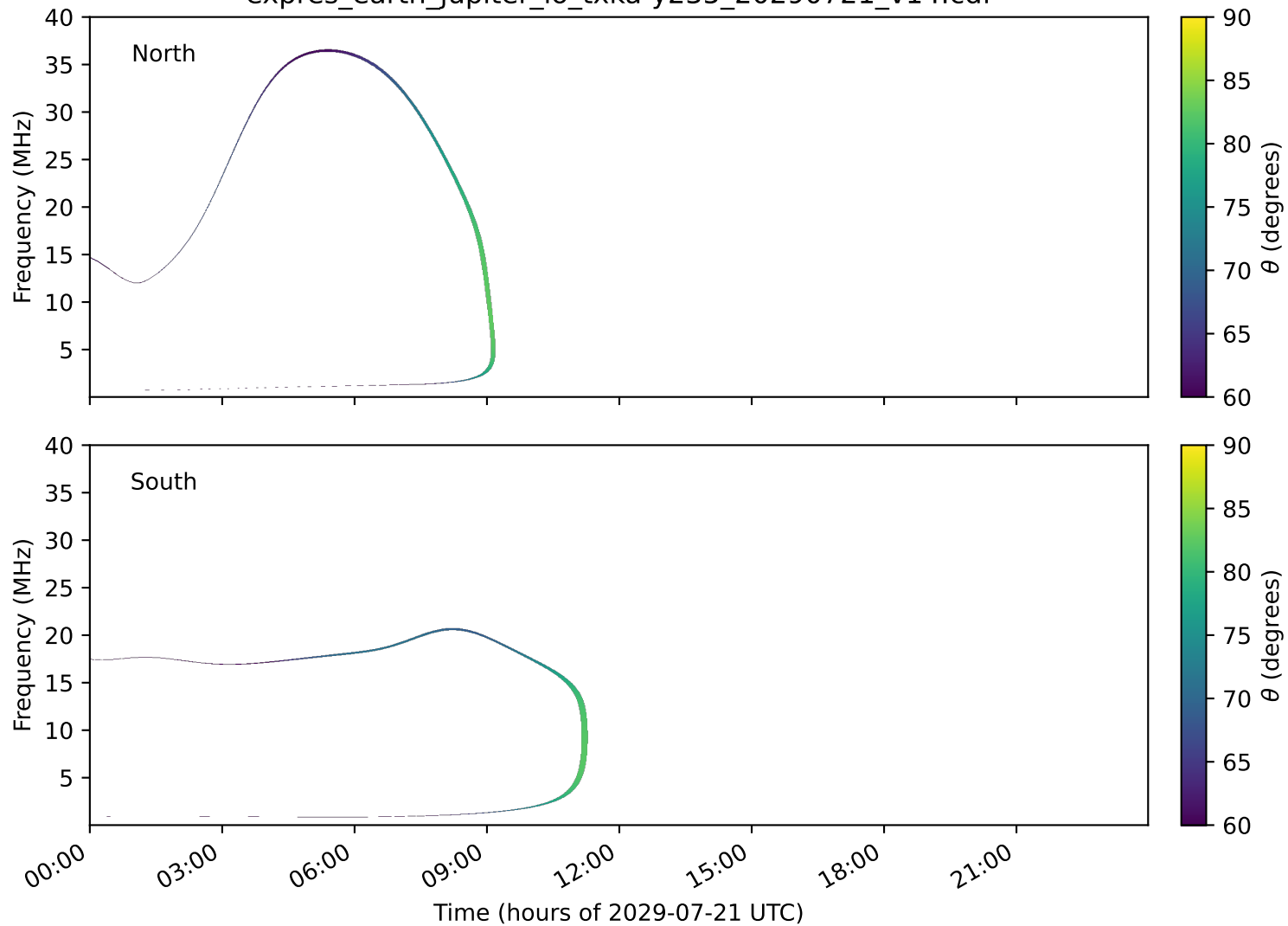
expres_earth_jupiter_io_txka-y235_20290721_v14.cdf
