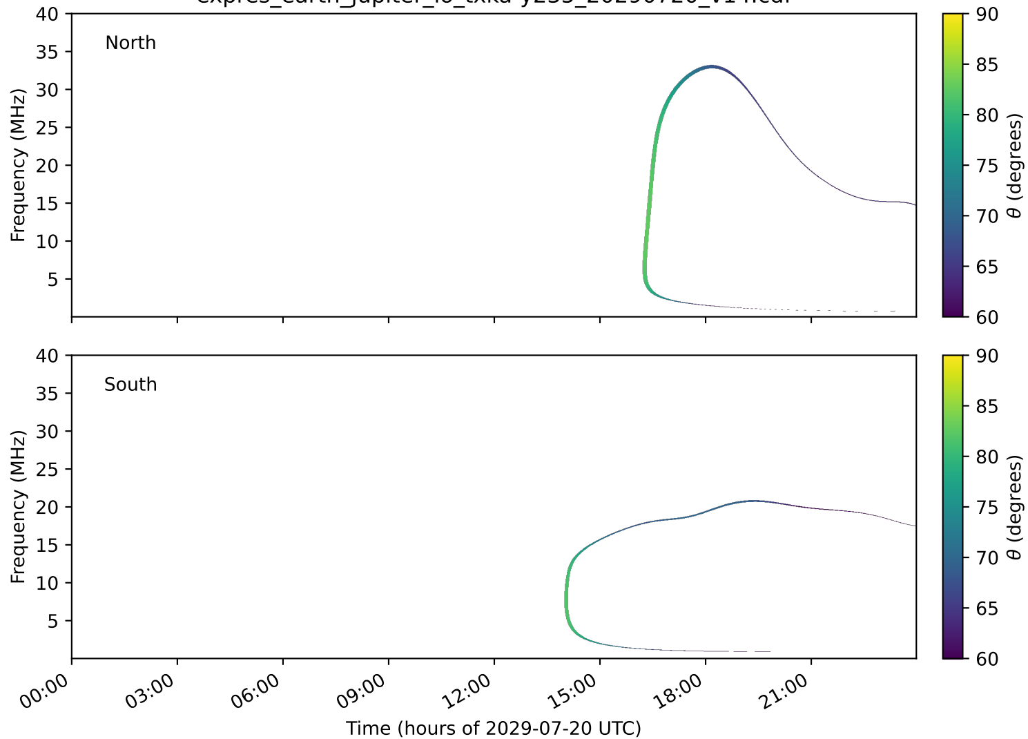
expres_earth_jupiter_io_txka-y235_20290720_v14.cdf
