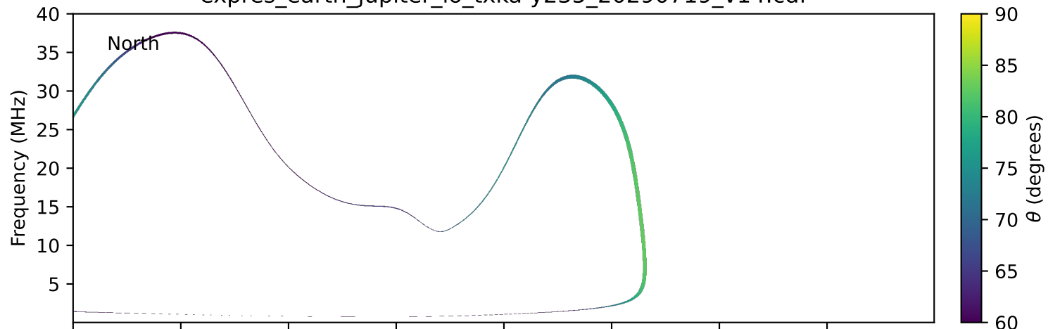
expres_earth_jupiter_io_txka-y235_20290719_v14.cdf
