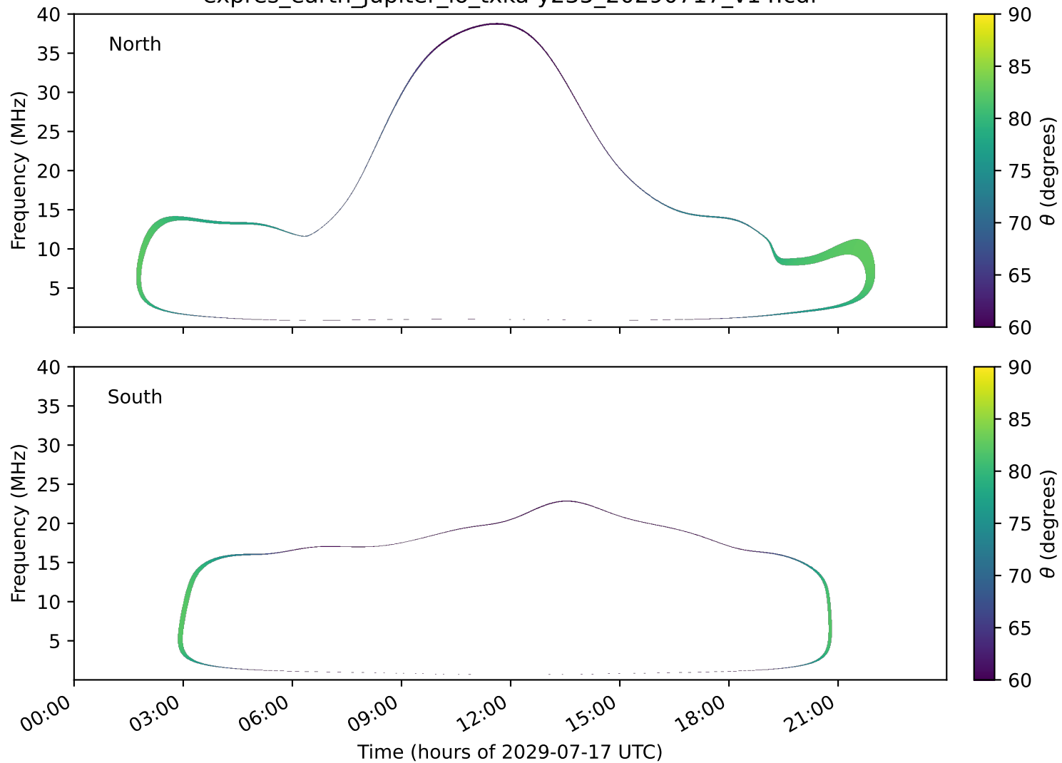
expres_earth_jupiter_io_txka-y235_20290717_v14.cdf
