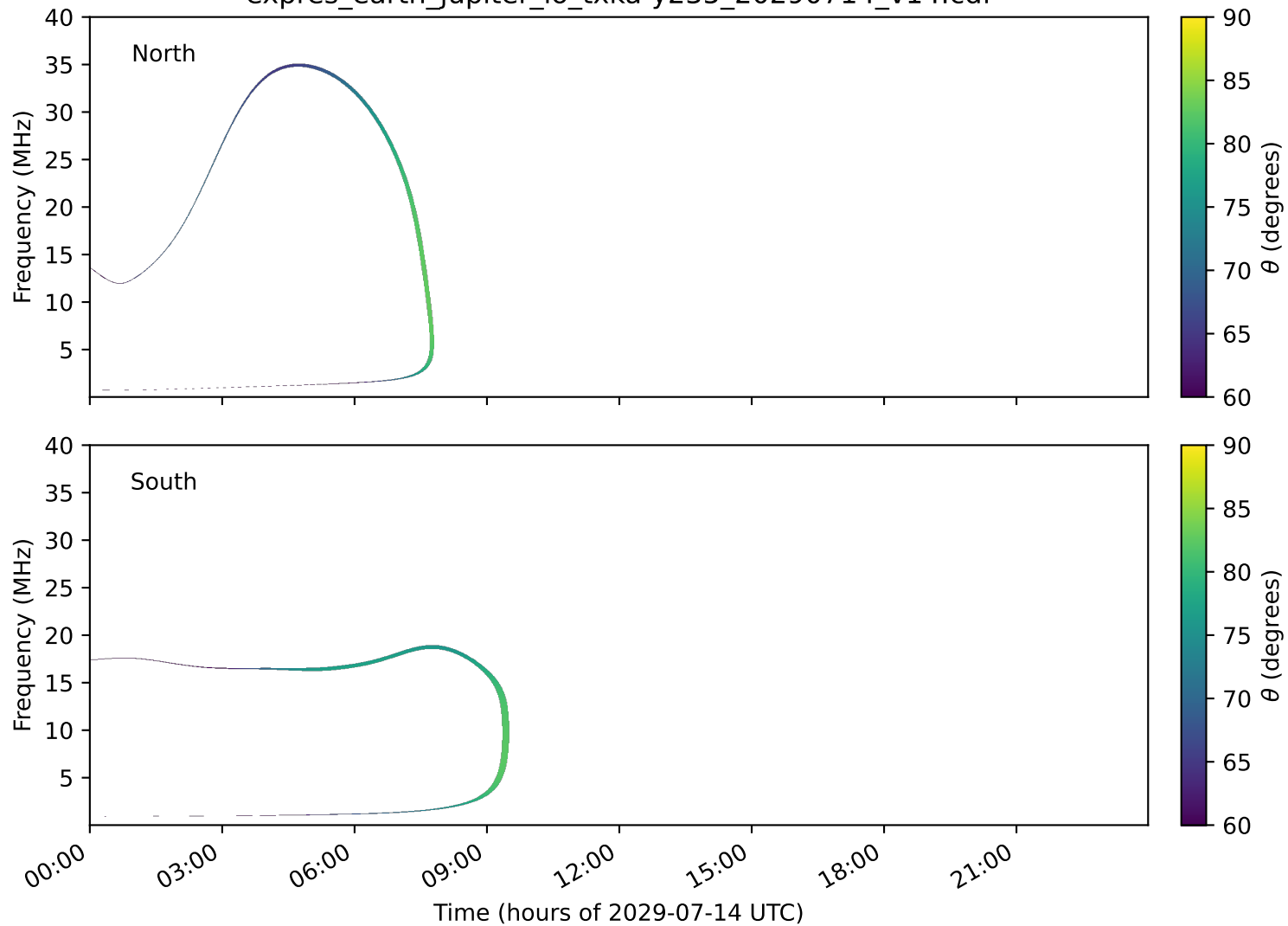
expres_earth_jupiter_io_txka-y235_20290714_v14.cdf
