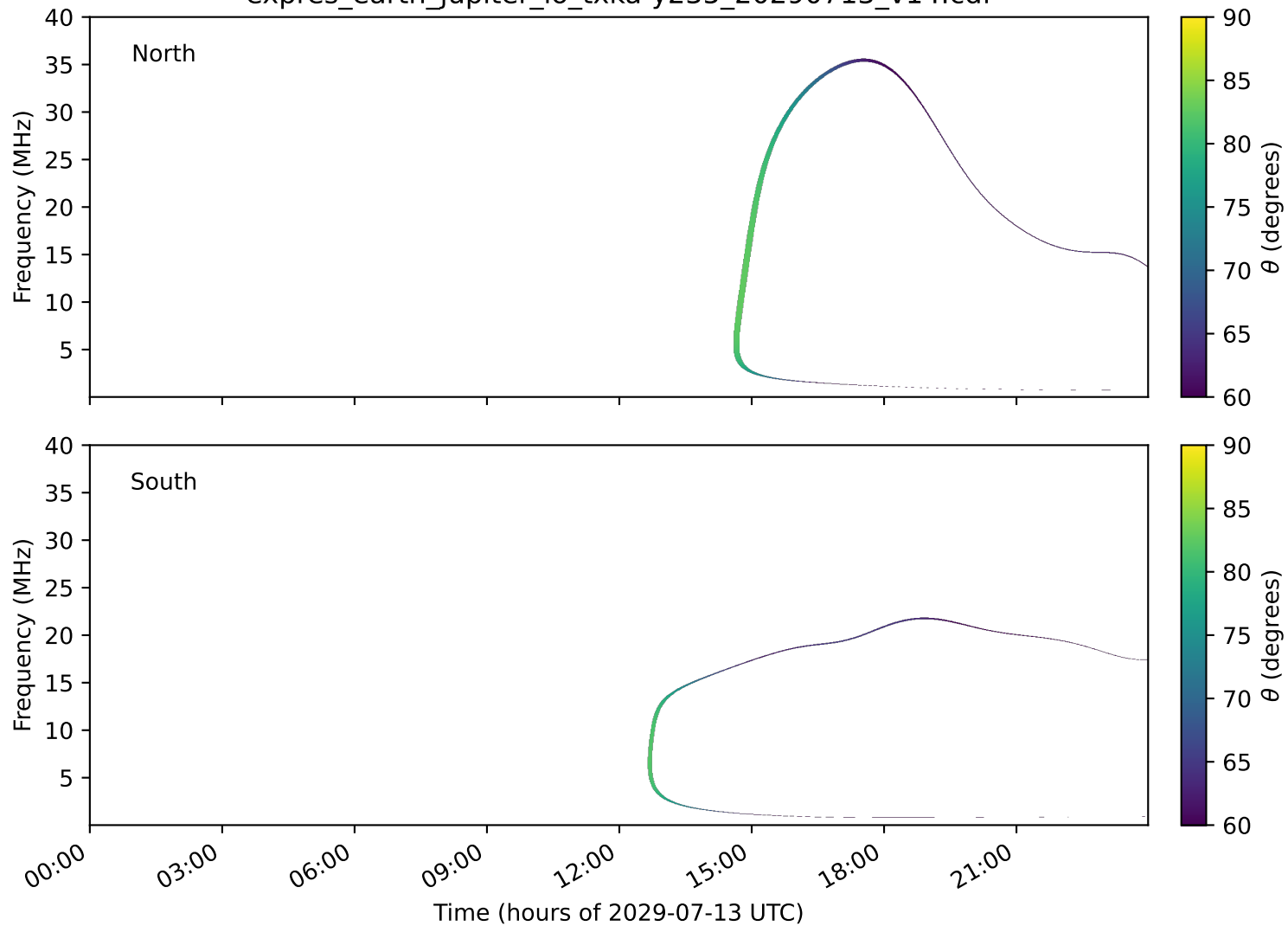
expres_earth_jupiter_io_txka-y235_20290713_v14.cdf
