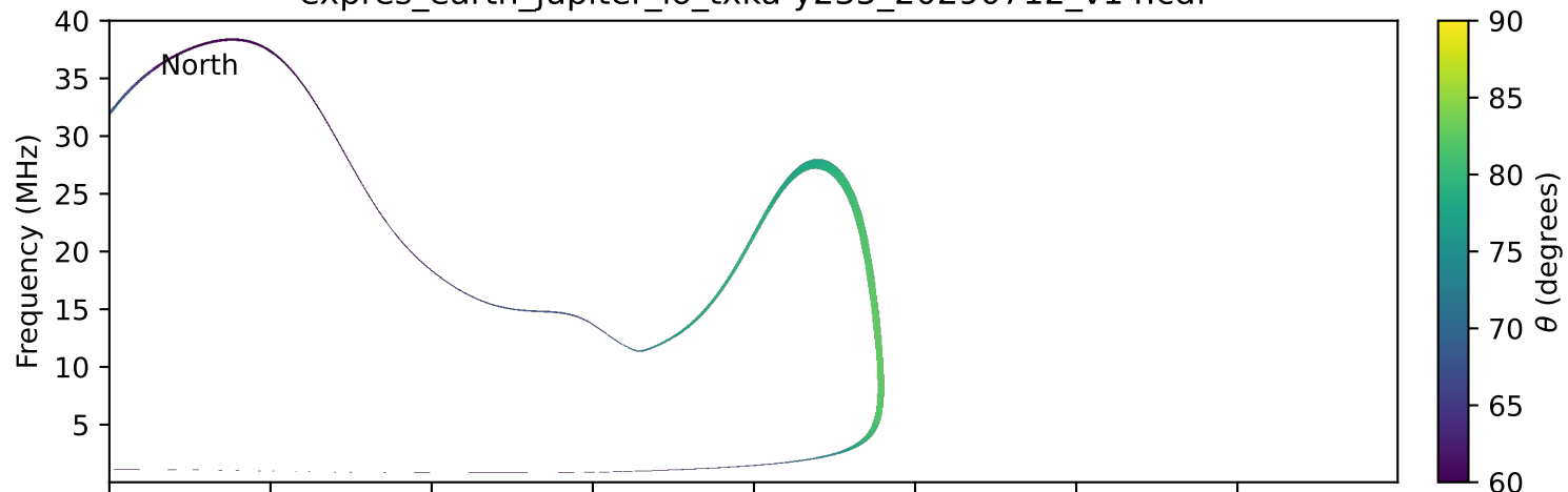
expres_earth_jupiter_io_txka-y235_20290712_v14.cdf
