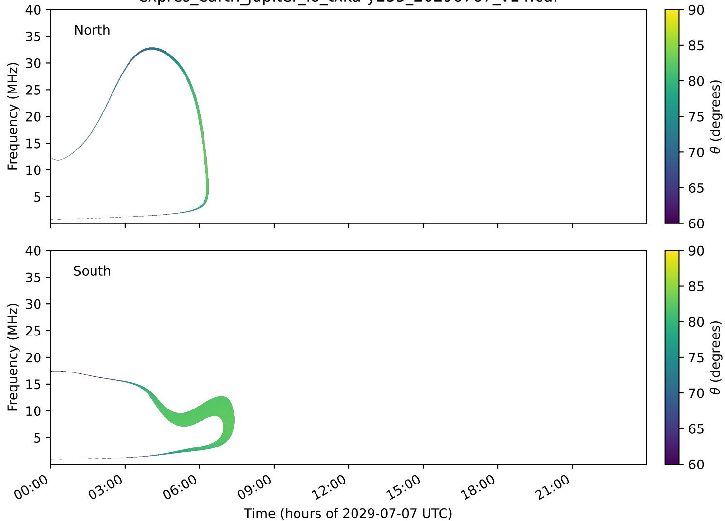
expres_earth_jupiter_io_txka-y235_20290707_v14.cdf
