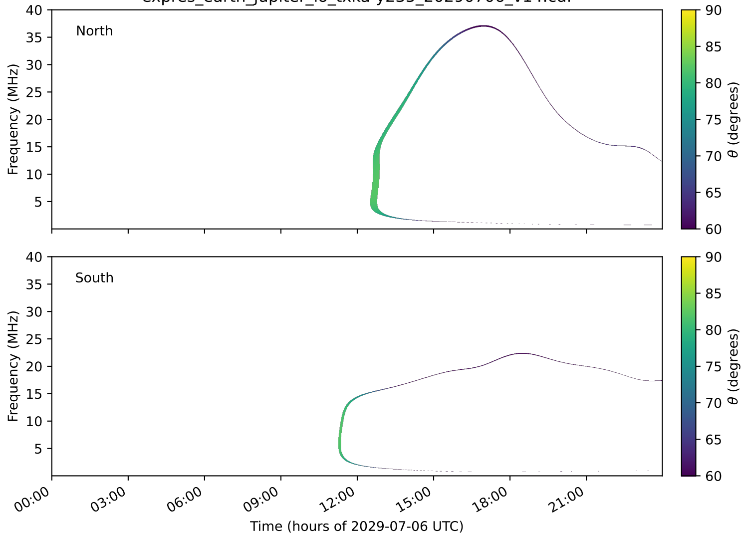
expres_earth_jupiter_io_txka-y235_20290706_v14.cdf
