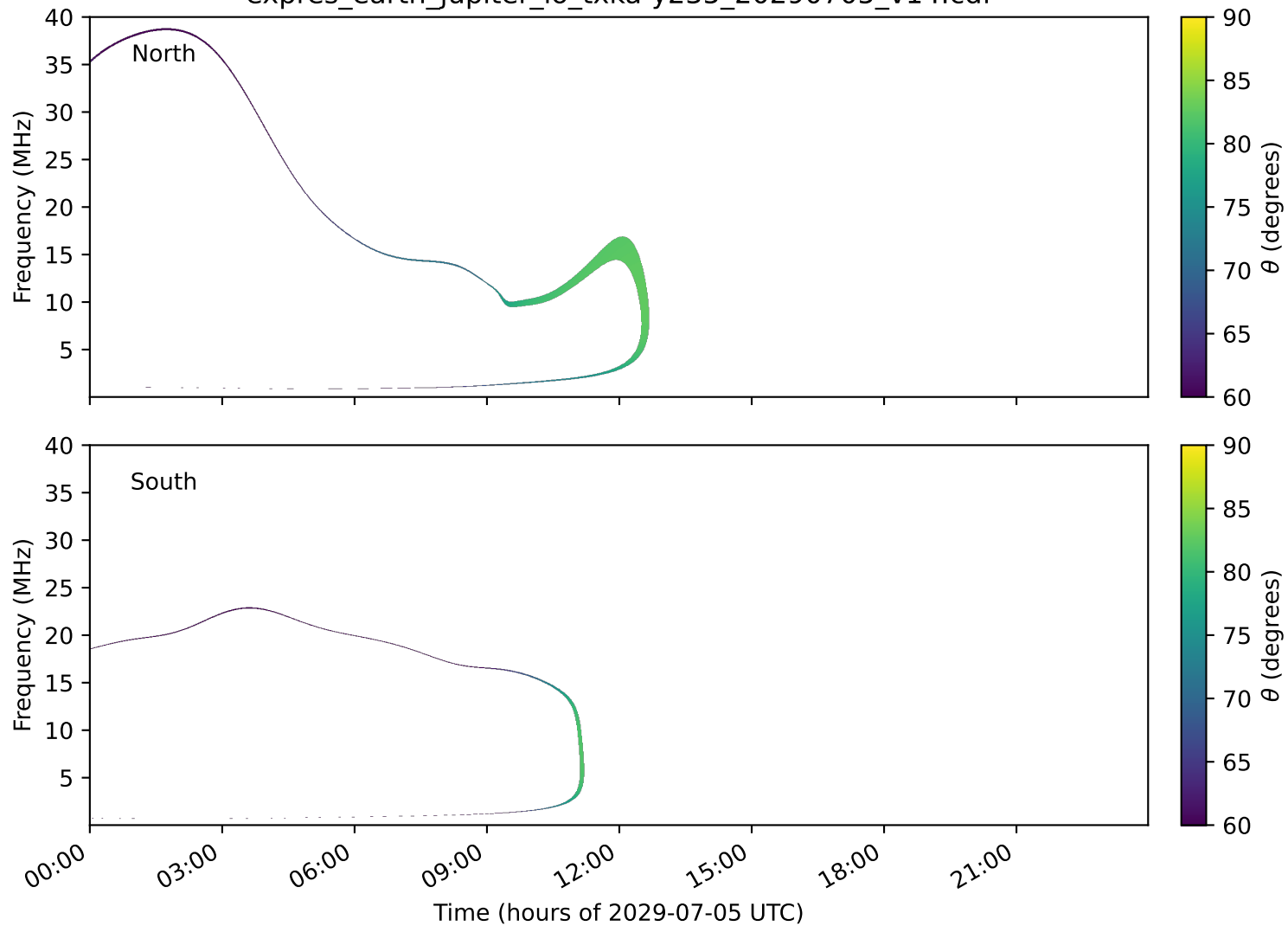
expres_earth_jupiter_io_txka-y235_20290705_v14.cdf
