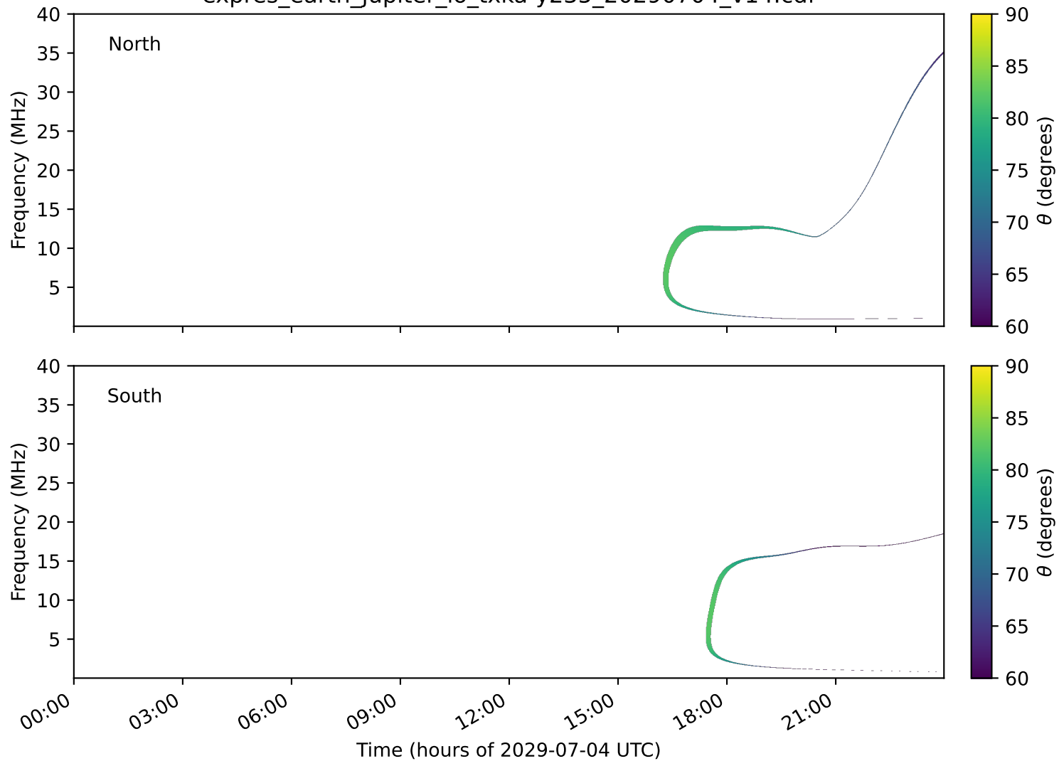
expres_earth_jupiter_io_txka-y235_20290704_v14.cdf
