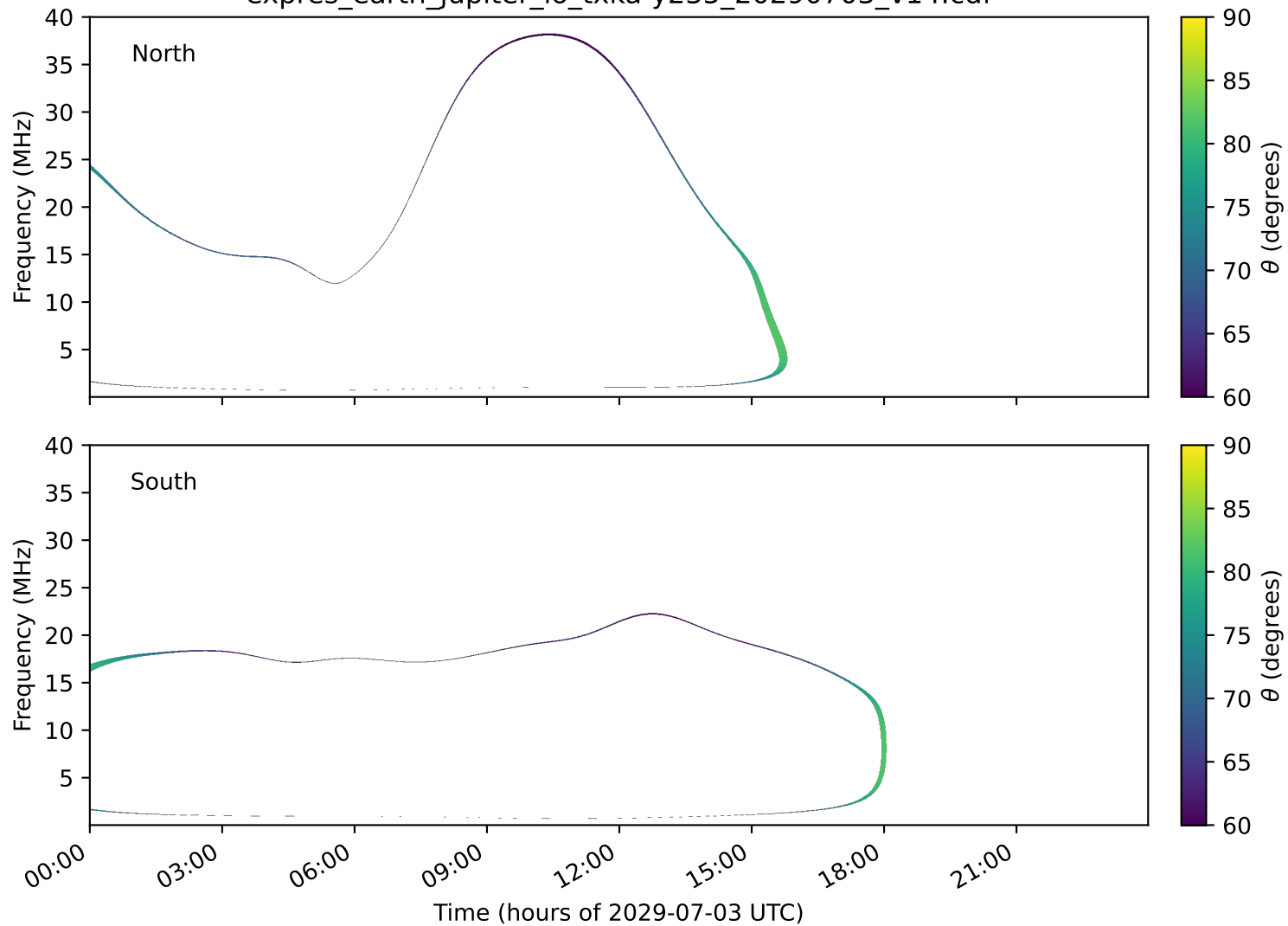
expres_earth_jupiter_io_txka-y235_20290703_v14.cdf
