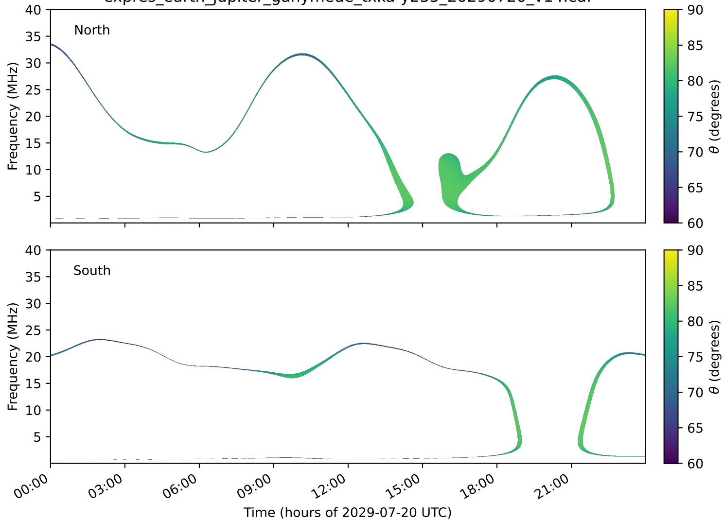
expres_earth_jupiter_ganymede_txka-y235_20290720_v14.cdf
