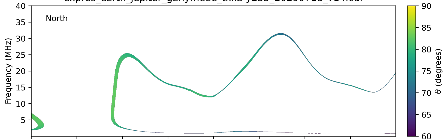
expres_earth_jupiter_ganymede_txka-y235_20290718_v14.cdf
