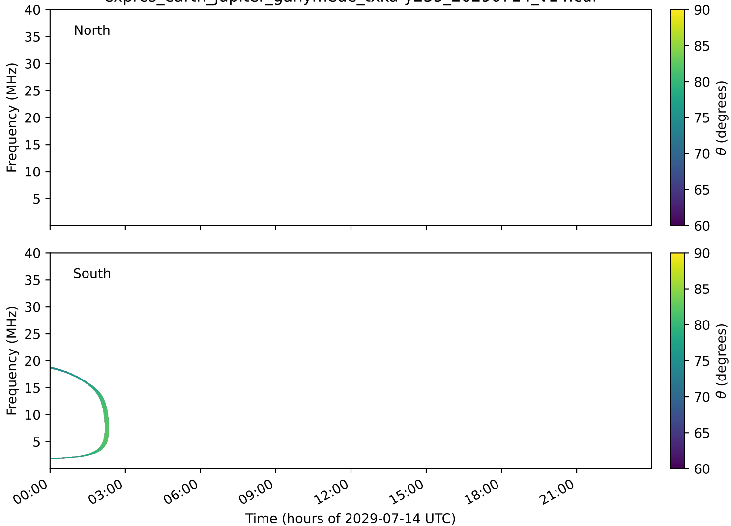
expres_earth_jupiter_ganymede_txka-y235_20290714_v14.cdf
