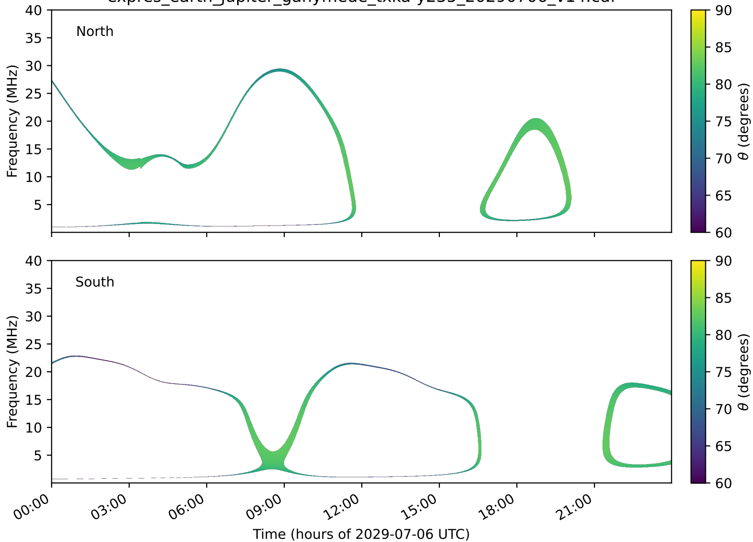
expres_earth_jupiter_ganymede_txka-y235_20290706_v14.cdf
