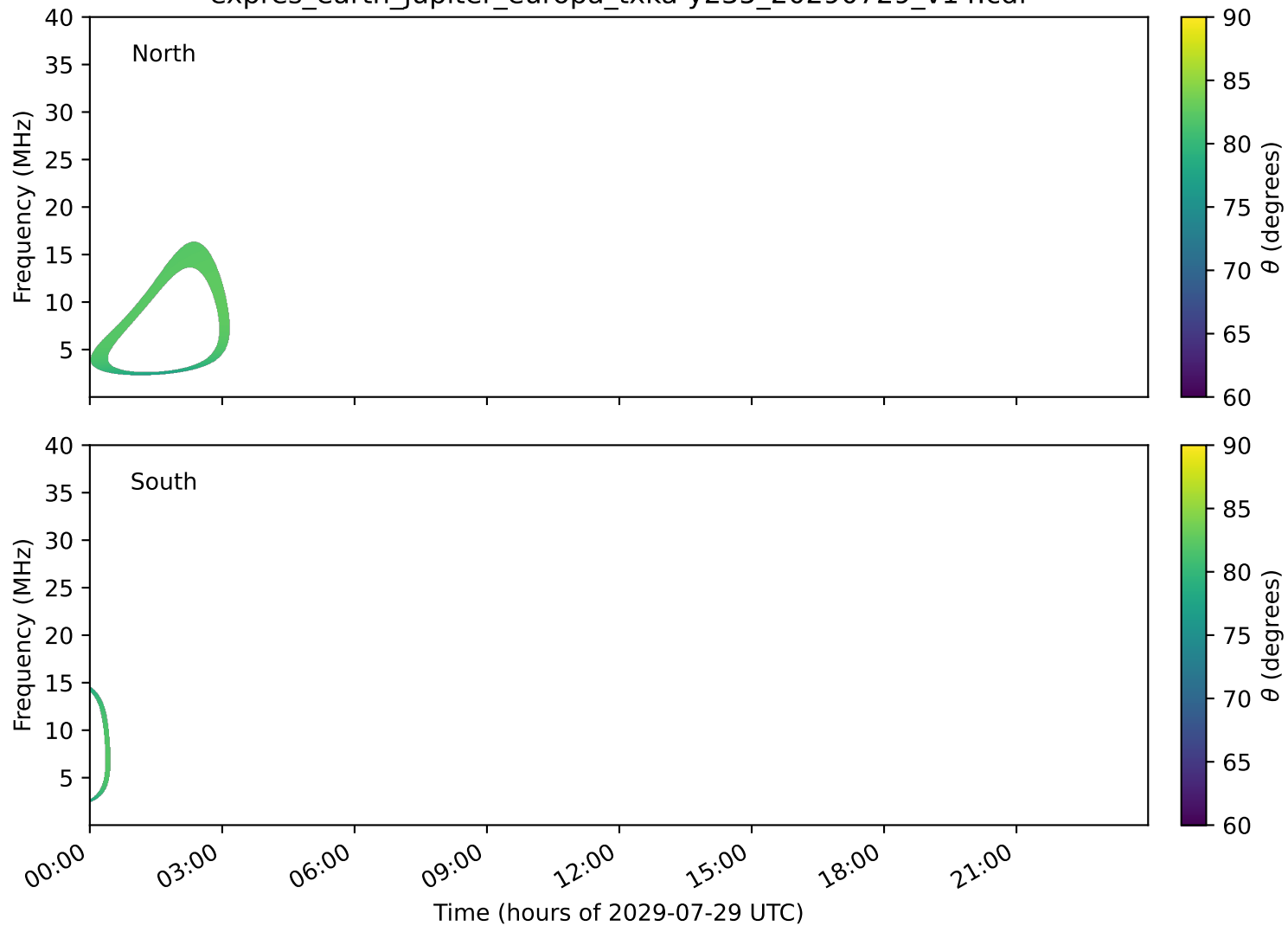
expres_earth_jupiter_europa_txka-y235_20290729_v14.cdf
