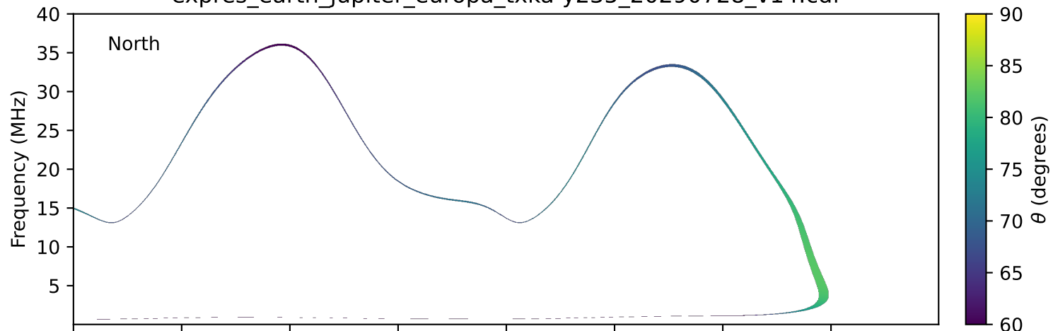
expres_earth_jupiter_europa_txka-y235_20290728_v14.cdf
