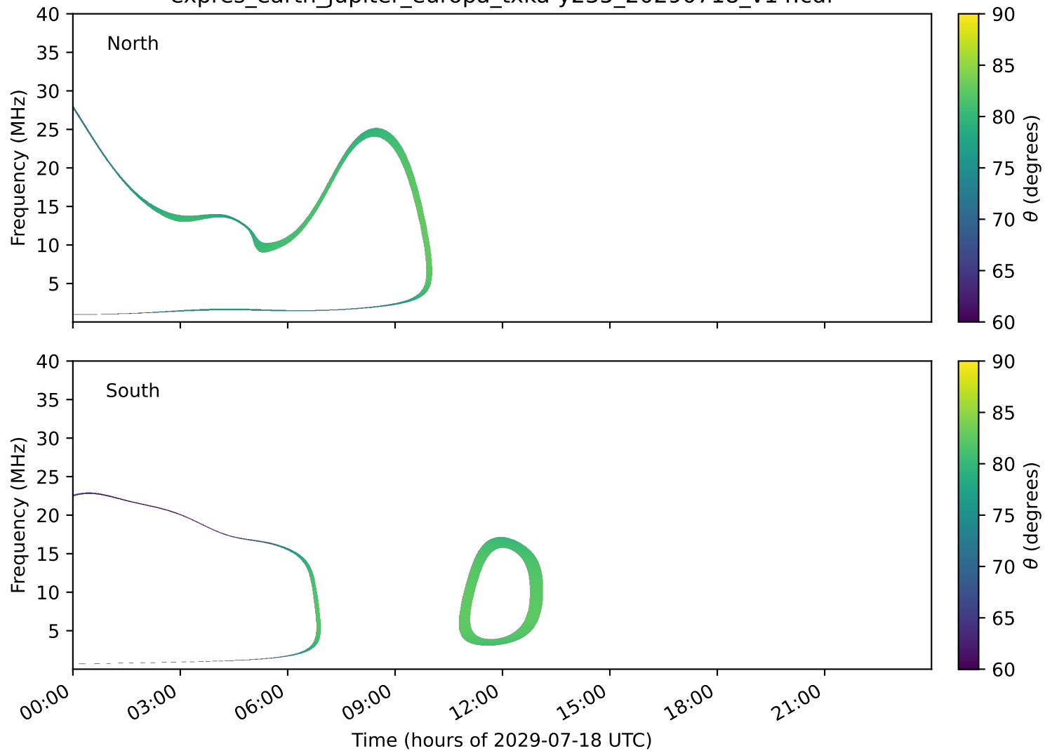
expres_earth_jupiter_europa_txka-y235_20290718_v14.cdf
