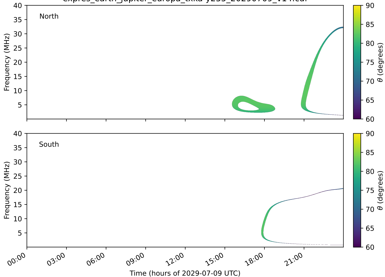
expres_earth_jupiter_europa_txka-y235_20290709_v14.cdf
