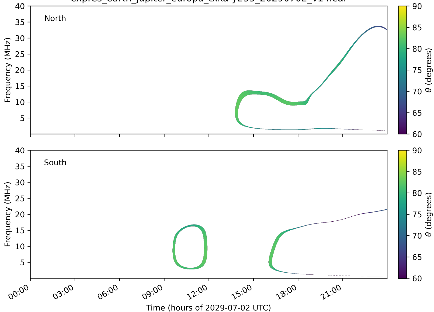
expres_earth_jupiter_europa_txka-y235_20290702_v14.cdf
