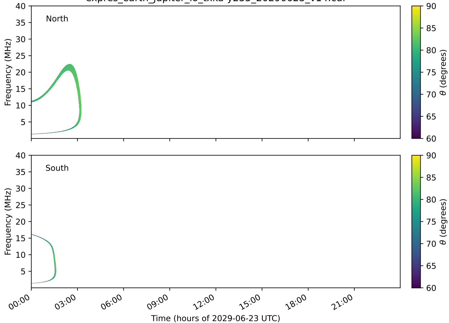
expres_earth_jupiter_io_txka-y235_20290623_v14.cdf
