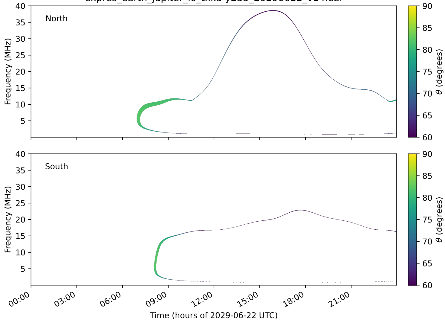
expres_earth_jupiter_io_txka-y235_20290622_v14.cdf
