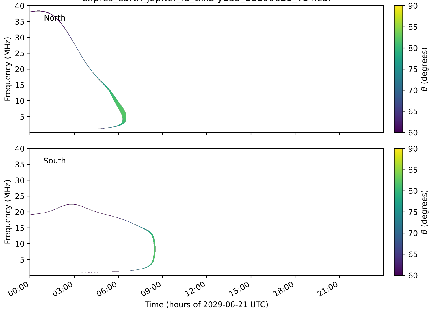
expres_earth_jupiter_io_txka-y235_20290621_v14.cdf
