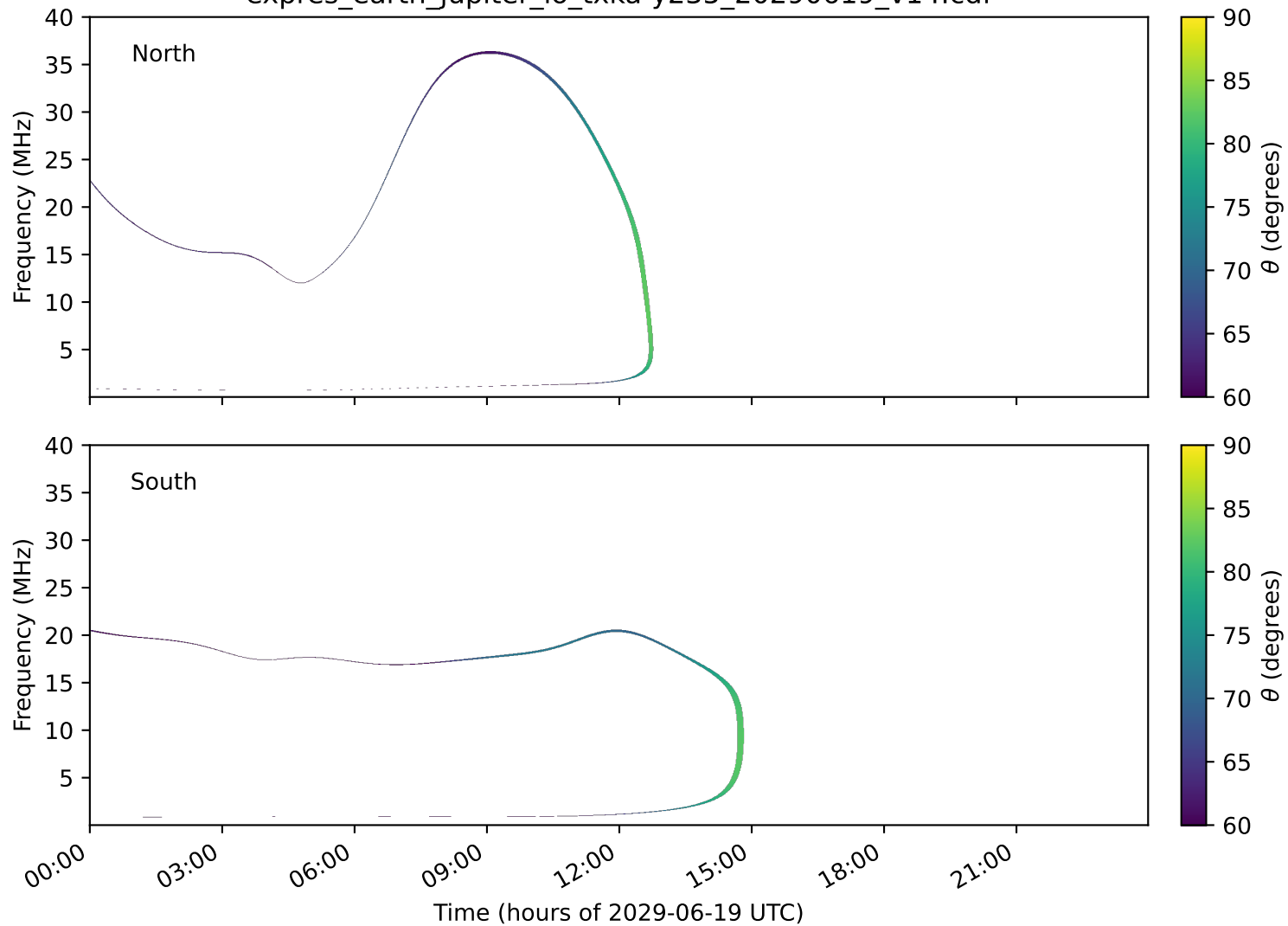
expres_earth_jupiter_io_txka-y235_20290619_v14.cdf
