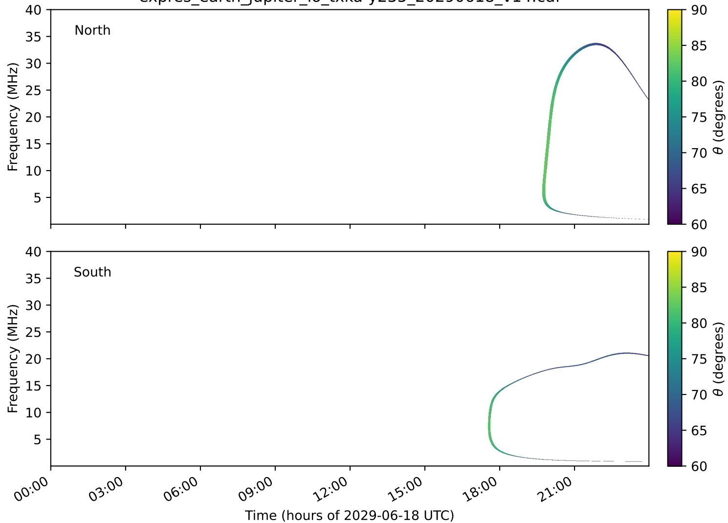
expres_earth_jupiter_io_txka-y235_20290618_v14.cdf
