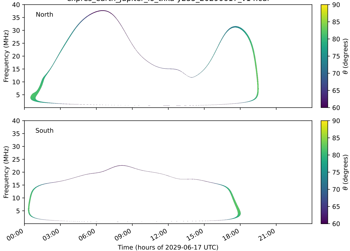
expres_earth_jupiter_io_txka-y235_20290617_v14.cdf
