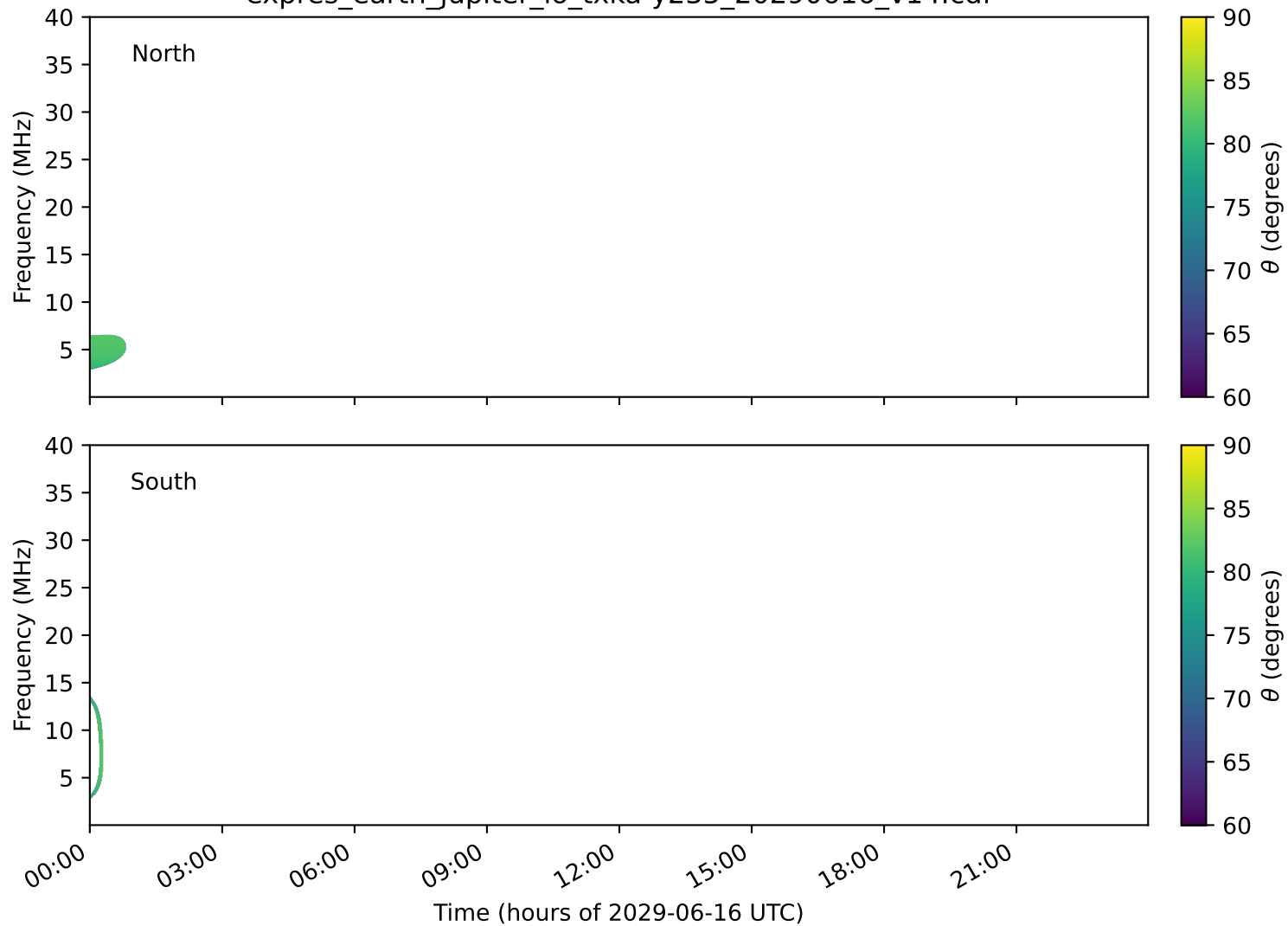
expres_earth_jupiter_io_txka-y235_20290616_v14.cdf
