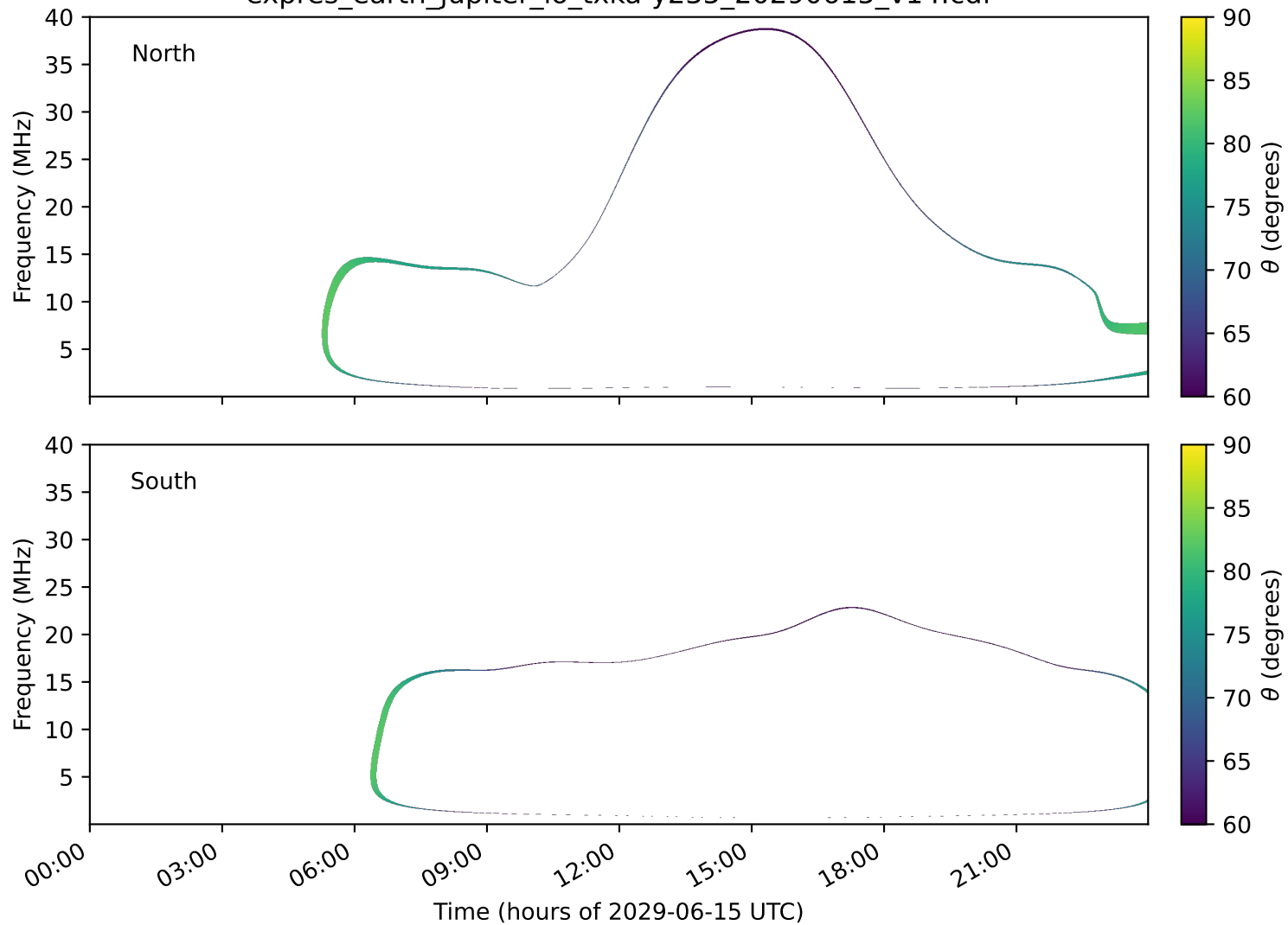
expres_earth_jupiter_io_txka-y235_20290615_v14.cdf
