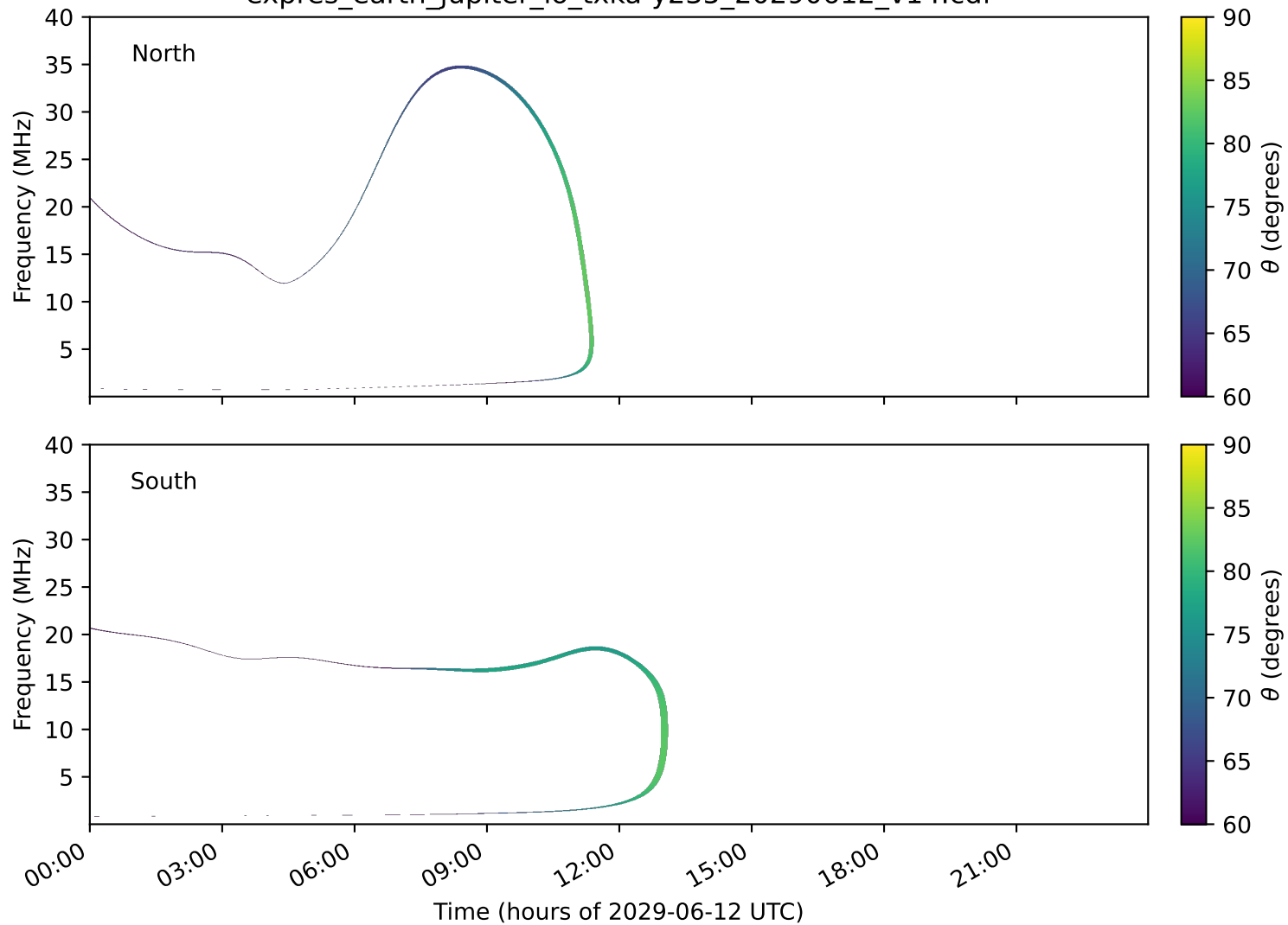
expres_earth_jupiter_io_txka-y235_20290612_v14.cdf
