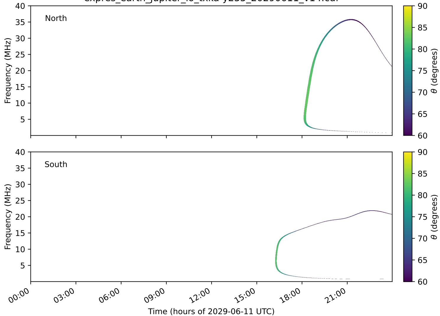
expres_earth_jupiter_io_txka-y235_20290611_v14.cdf
